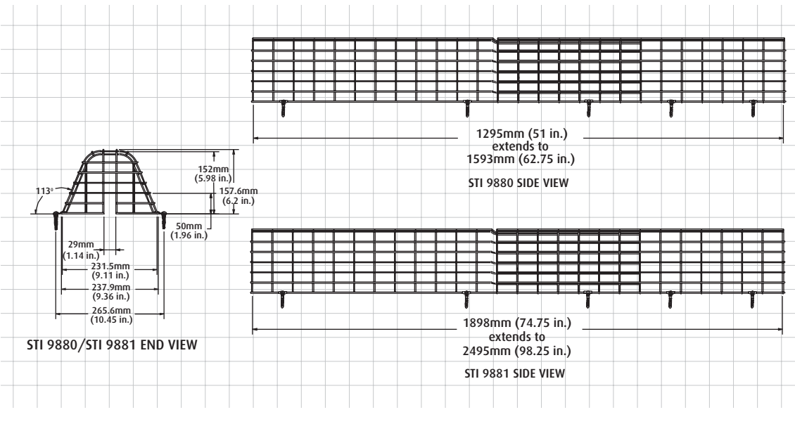
▼ Fluorescent Light Cage dimensions and technical information (STI 9880 & STI 9881)
